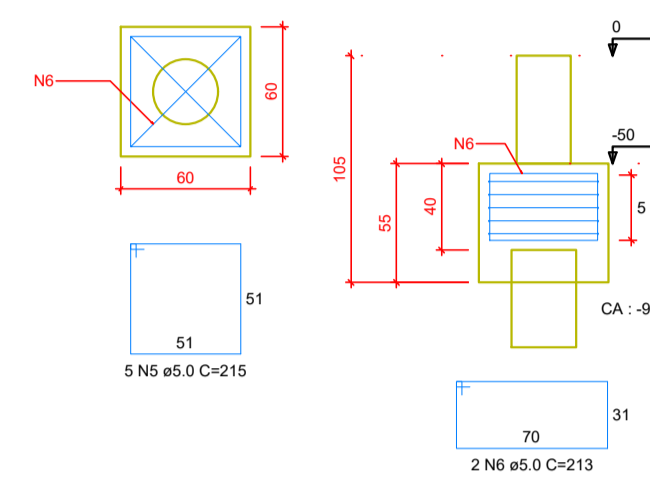
B1=B2=B3=B4=B5=B8=B9=B14=B15=B20=B21 =B26=B33=B34=B37=B38=B39=B40=B41 1xC30 PLANTA ESC 1:25
